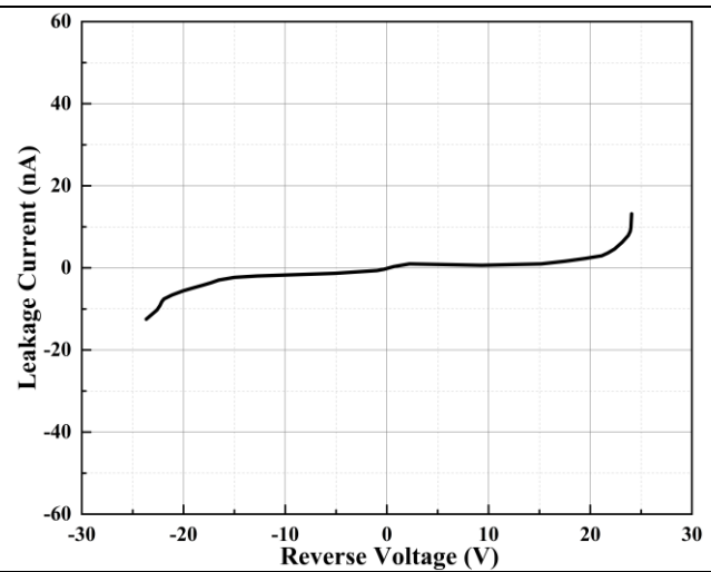
Figure 2. Leakage Current vs. Reverse Voltage
