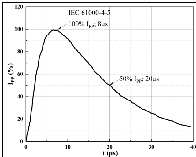
Figure 6. 8/20 \mu s Pulse Waveform
