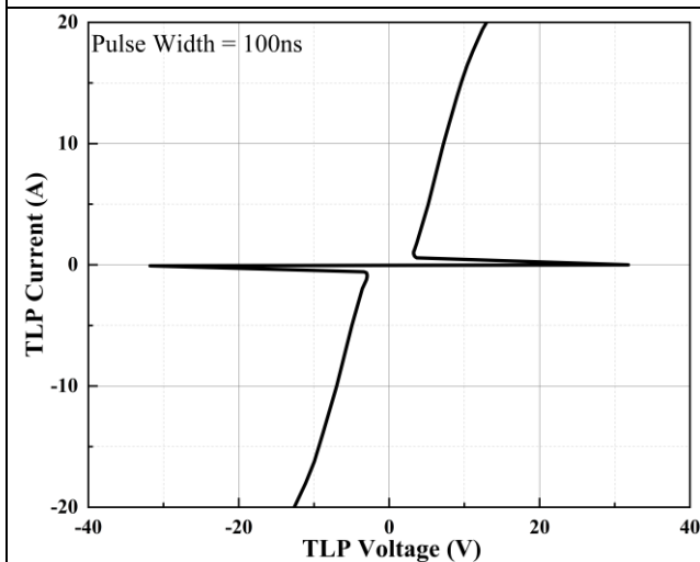
Figure 5. TLP Current vs. TLP Voltage
