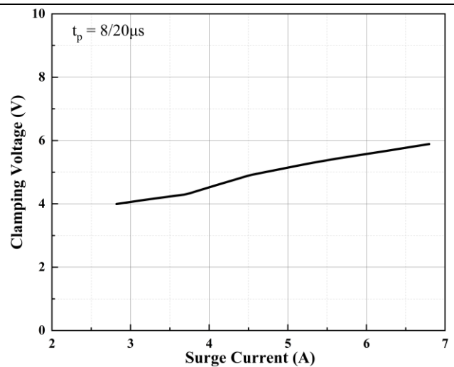
Figure 4. Clamping Voltage vs. Surge Current
