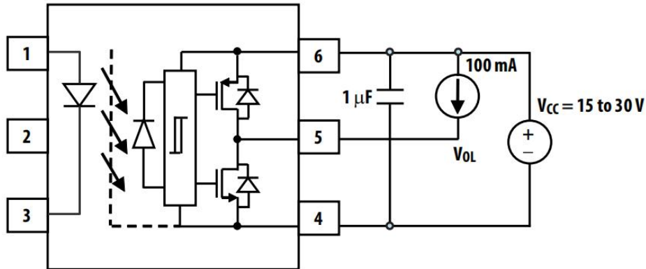
Fig.20 Test Circuits for V_{OL}
