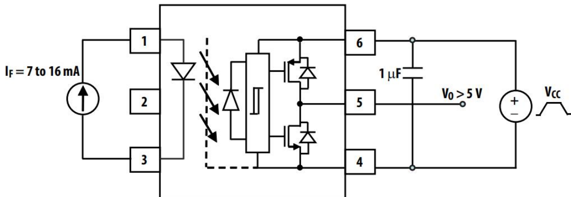
Fig.22 Test Circuits for UVLO
