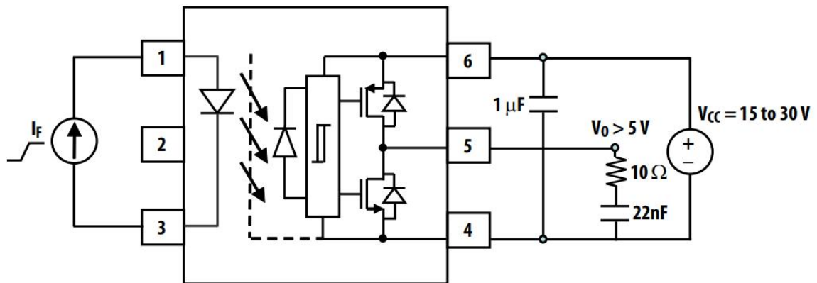
Fig.21 Test Circuits for I_{FHL}
