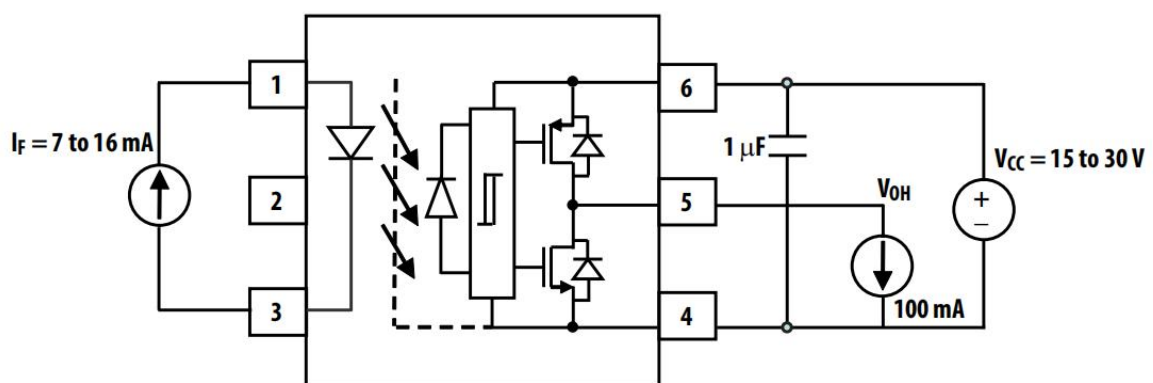
Fig.19 Test Circuits for V_{OH}
