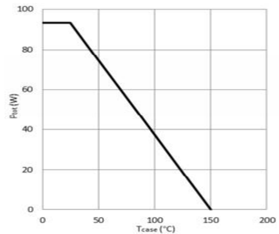
Figure 12. Power Dissipation
