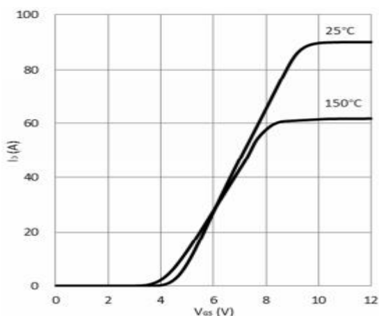
Figure 3. Typical Transfer Characteristics V_{DS}=10\text{V} Parameter: T_J
