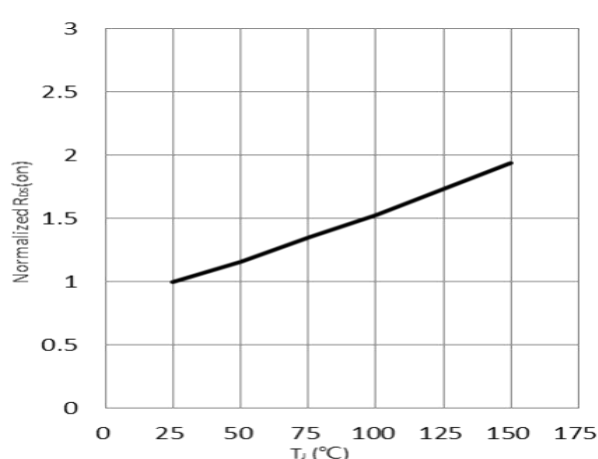
Figure 4. Normalized On-resistance I_D = 4\text{ A}, V_{GS} = 12\text{ V}
