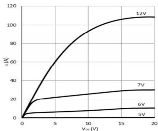
Figure 1. Typical Output Characteristics T_J=25^\circ\text{C} Parameter: V_{GS}
