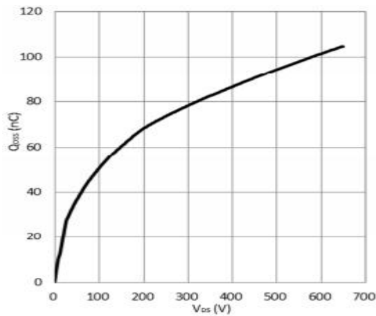
Figure 7. Typical Q_{oss}
