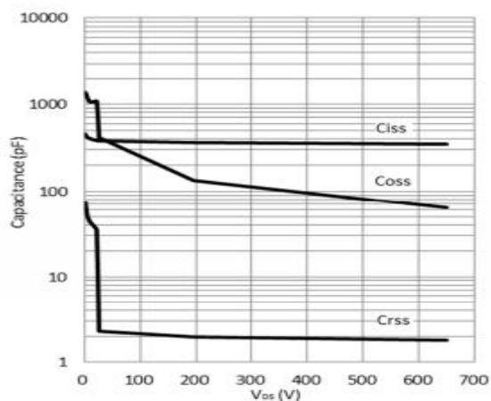
Figure 5. Typical Capacitance V_{GS} = 0\text{V}, f = 1\text{MHz}
