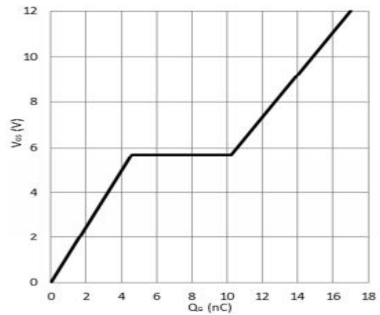
Figure 8. Typical Gate Charge
