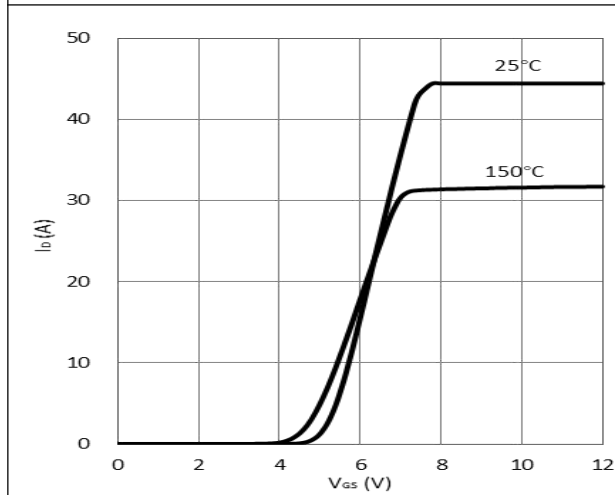
Figure 3. Typical Transfer Characteristics V_{DS}=10\text{V} Parameter: T_j
