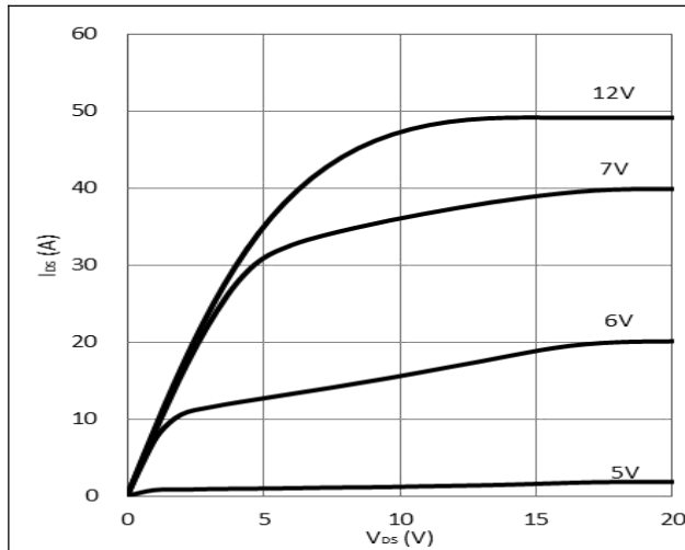
Figure 1. Typical Output Characteristics T_j=25^\circ\text{C} Parameter: V_{GS}
