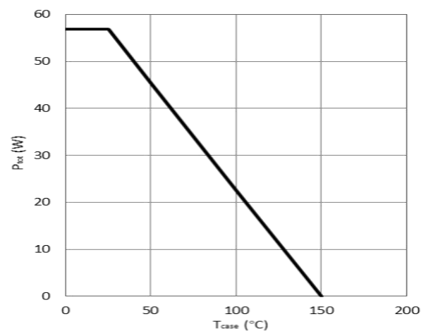
Figure 12. Power Dissipation
