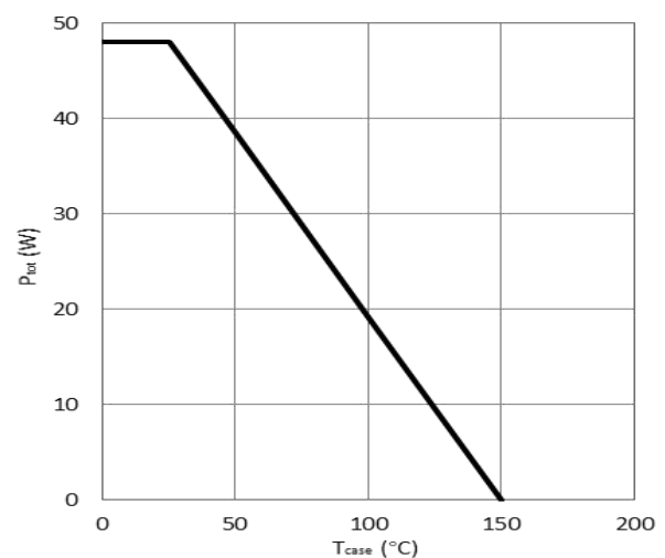
Figure 12. Power Dissipation
