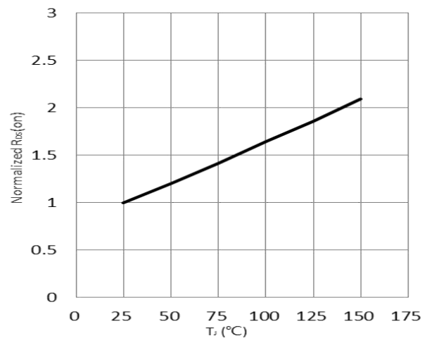
Figure 4. Normalized On-resistance I_D = 4\text{ A}, V_{GS} = 8\text{ V}
