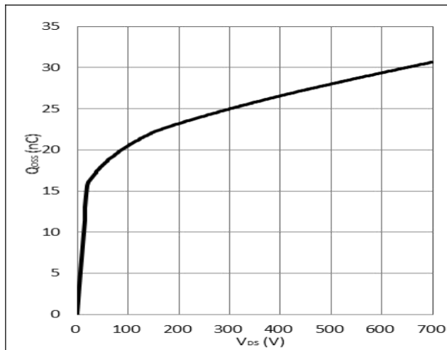
Figure 7. Typical Q_{oss}
