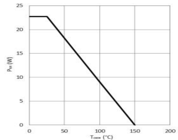
Figure 12. Power Dissipation
