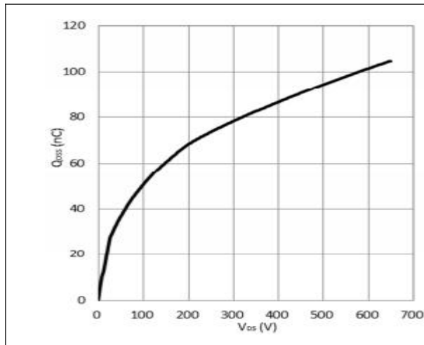
Figure 7. Typical Q_{oss}
