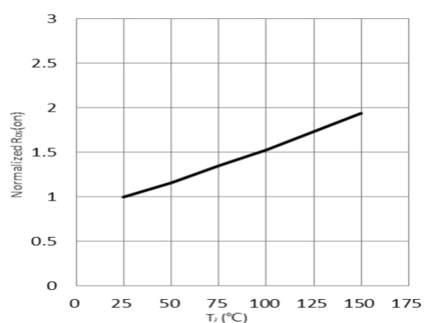
Figure 4. Normalized On-resistance I_D = 4\text{ A}, V_{GS} = 12\text{ V}
