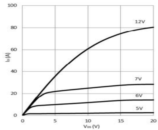
Figure 2. Typical Output Characteristics T_j = 150^\circ\text{C} Parameter: V_{GS}
