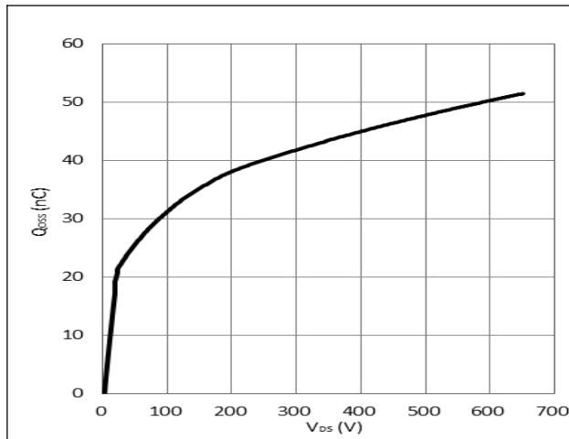
Figure 7. Typical Q_{oss}
