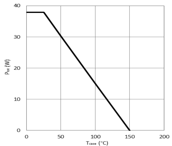
Figure 12. Power Dissipation
