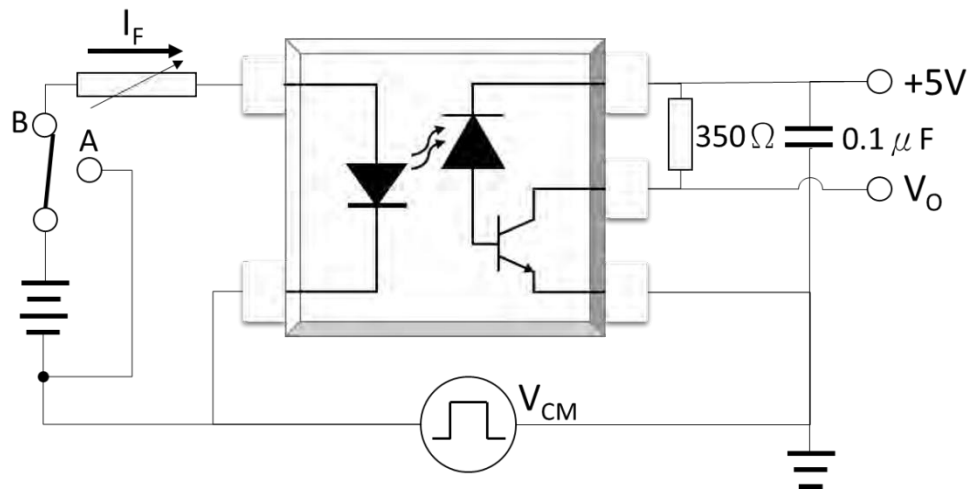
Fig.15 Test Circuits for Common Mode Transient Immunity
