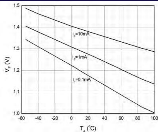
Fig.2 Forward Voltage vs. Ambient Temperature
