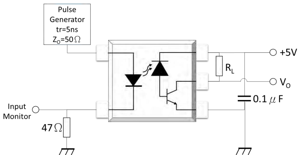
Fig.13 Test Circuits for TPHL, TPLH, tr, tf
