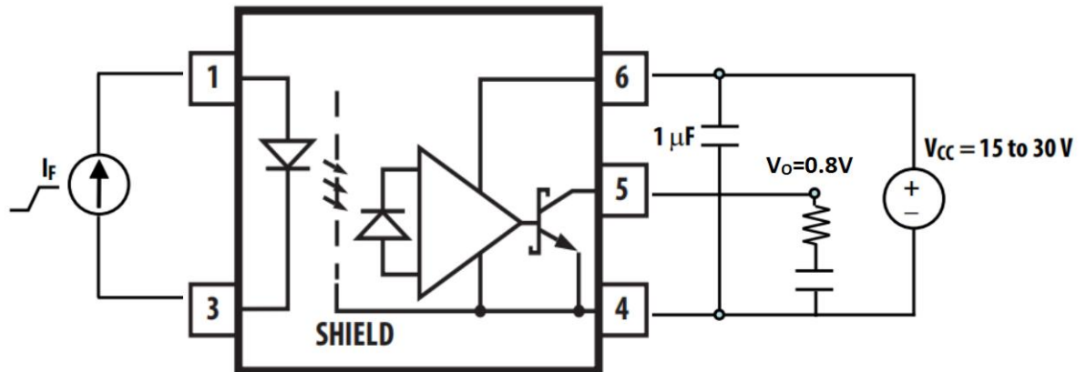
Fig.17 Test Circuits for ITH
