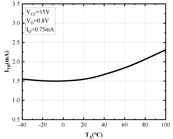
Fig.10 Input Threshold Current vs. Ambient Temperature
