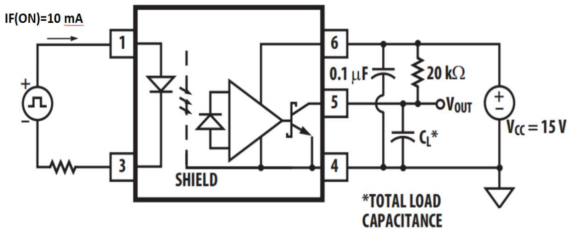
Fig.18 Test Circuits for TPHL, TPLH
