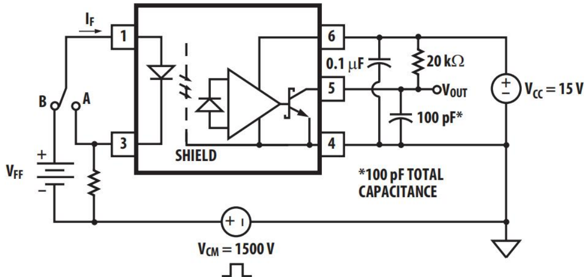
Fig.20 Test Circuits for Common Mode Transient Immunity
