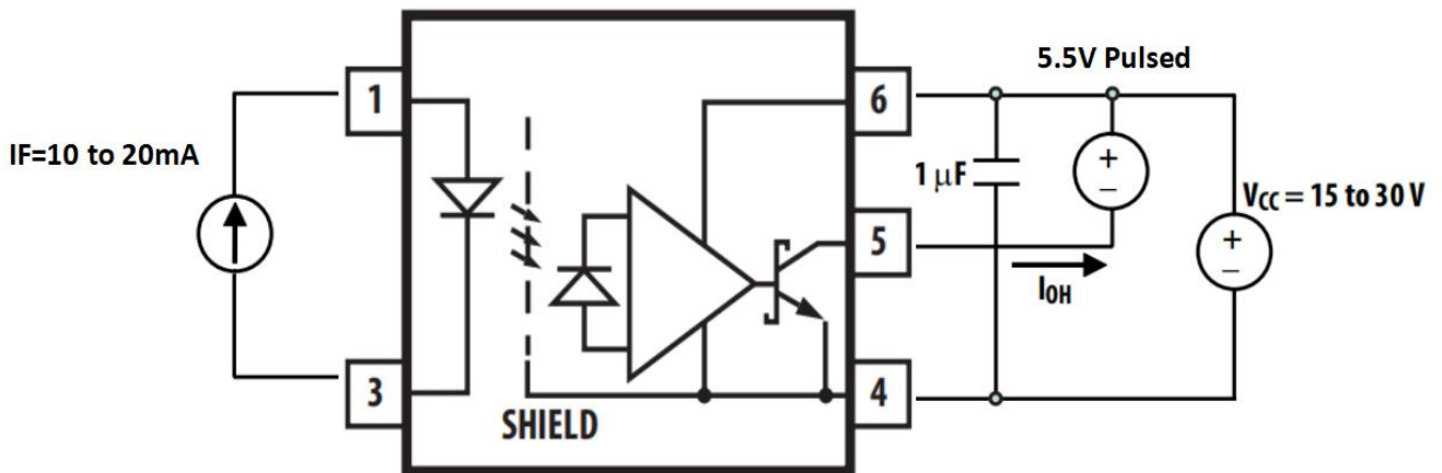
Fig.14 Test Circuits for I_{OH}
