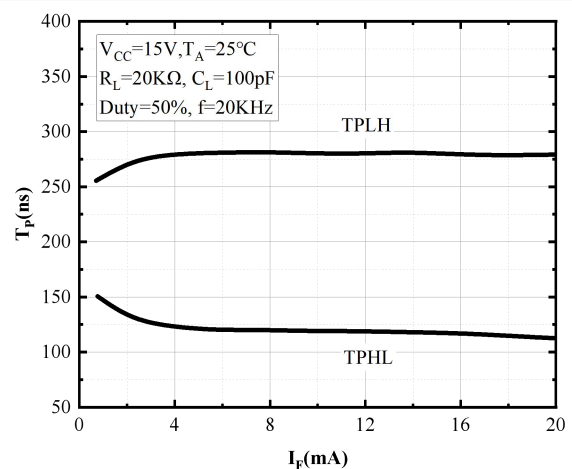
Fig.12 Propagation Delay vs. Forward Current
