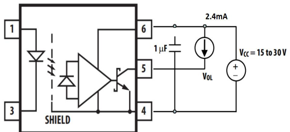
Fig.16 Test Circuits for V_{OL}
