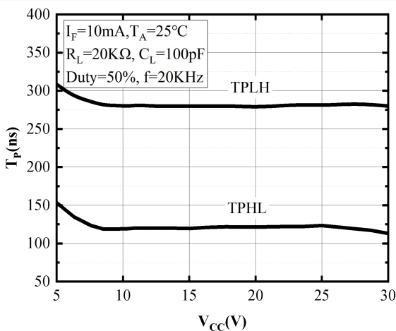
Fig.11 Propagation Delay vs. Supply Voltage
