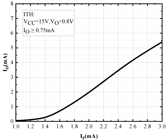
Fig.9 Output Current vs. Input Current
