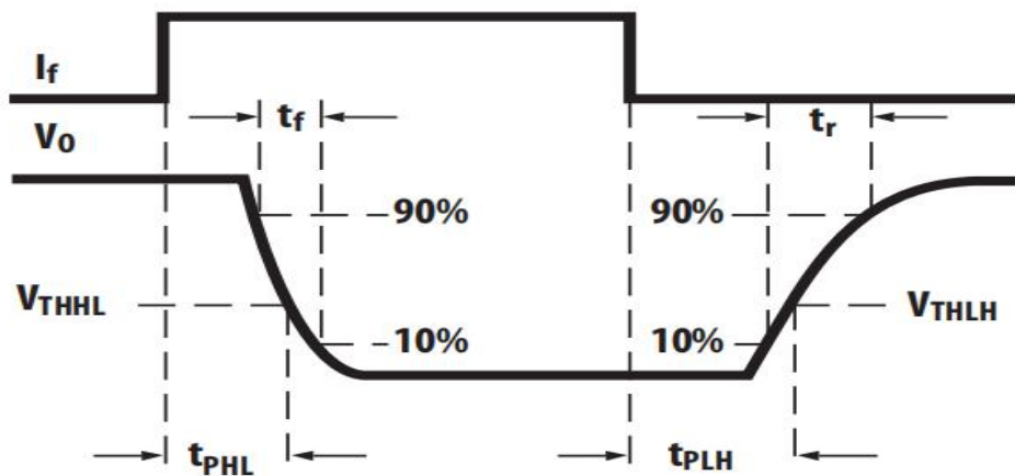
Fig.19 Wave forms of TPHL, TPLH
