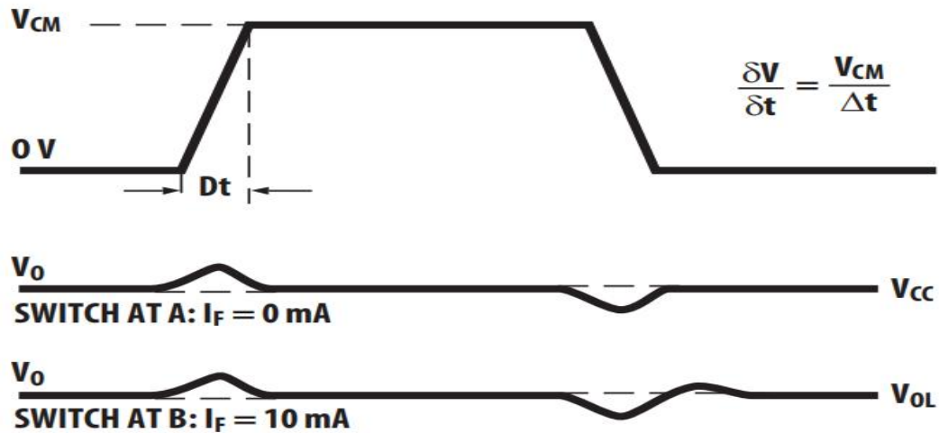
Fig.21 Waveforms of Common Mode Transient Immunity
