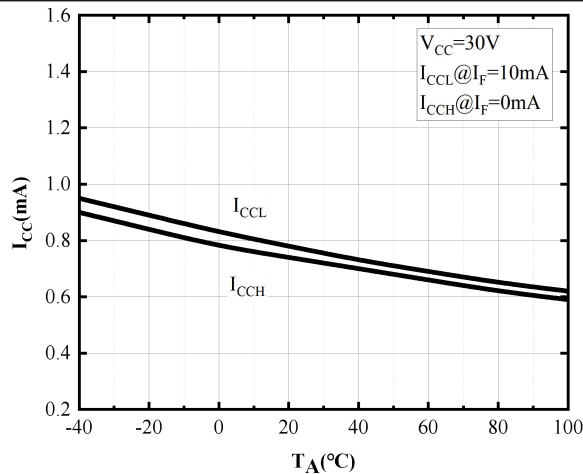
Fig.3 Supply Current vs. Ambient Temperature
