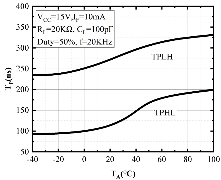
Fig.13 Propagation Delay vs. Ambient Temperature
