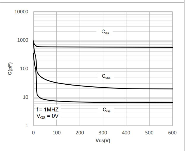
Figure 6. Capacitance Characteristics
