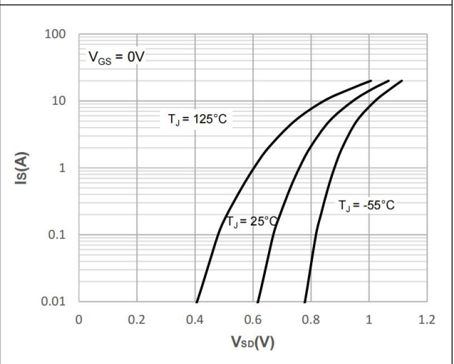
Figure 4. Body-Diode Characteristics
