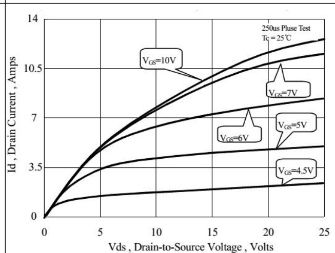
Figure 6. On-State Characteristics
