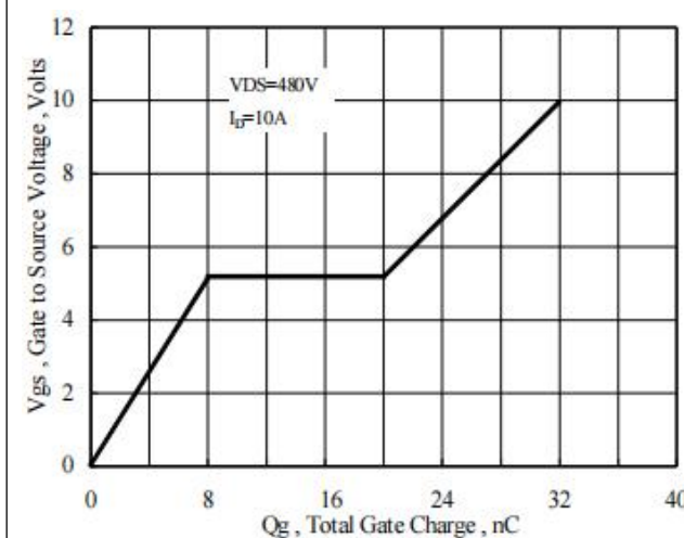
Figure 5. Gate-Charge Characteristics
