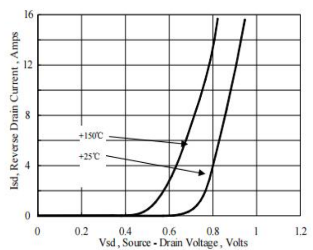
Figure 4. Body-Diode Characteristics
