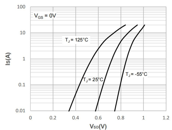
Figure 4. Body-Diode Characteristics
