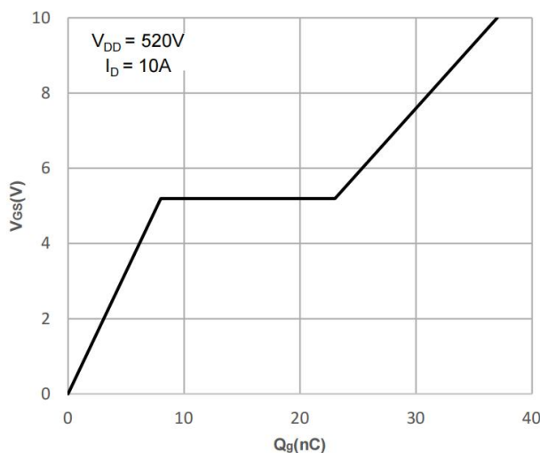
Figure 5. Gate-Charge Characteristics
