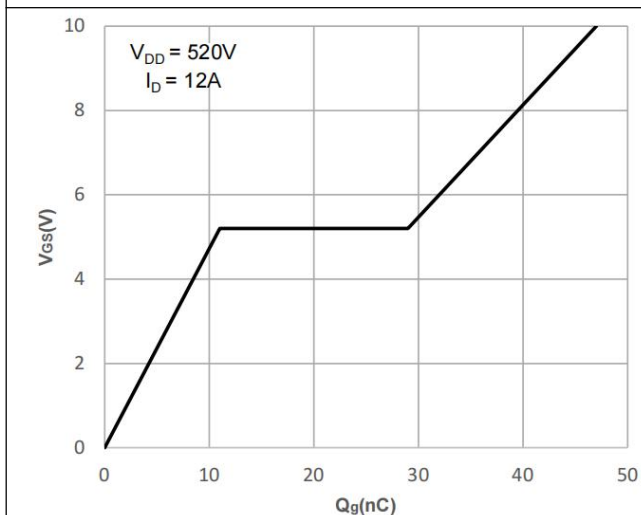
Figure 5. Gate-Charge Characteristics
