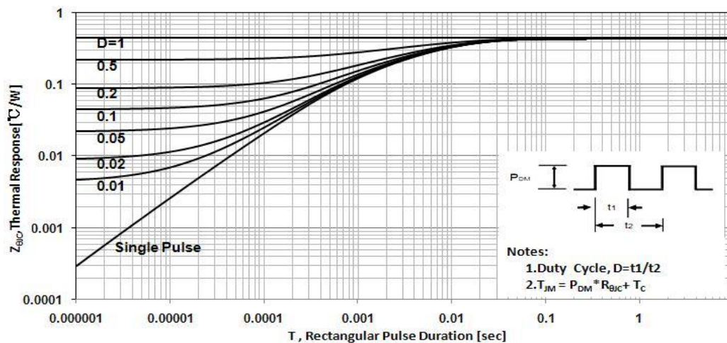
Figure 11. Normalized Effective Transient Thermal Impedance With Pulse Duration
