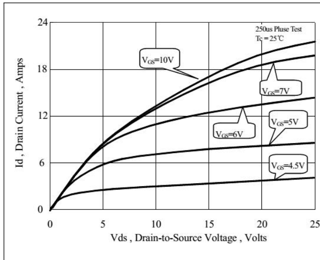
Figure 1. On-State Characteristics
