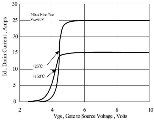
Figure 7. Transfer Characteristics Variation with Source Current
