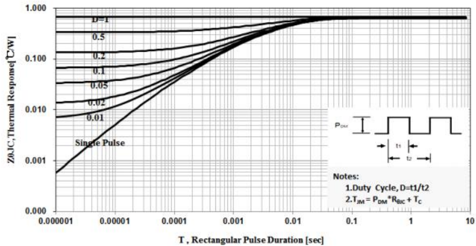
Figure 9. Normalized Effective Transient Thermal Impedance With Pulse Duration(TO-220)
