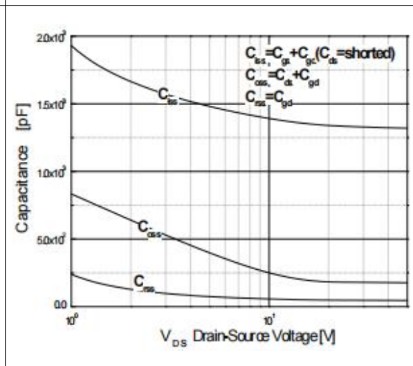
Figure 6. Capacitance Characteristics
