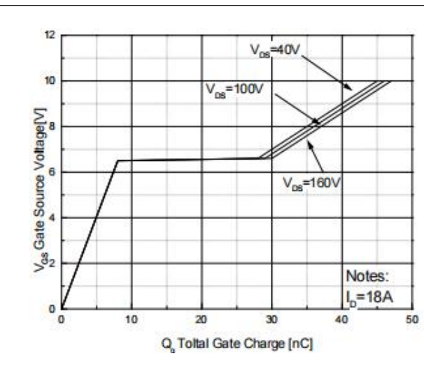
Figure 5. Gate-Charge Characteristics
