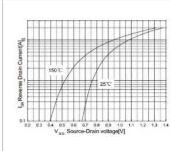
Figure 4. Body-Diode Characteristics
