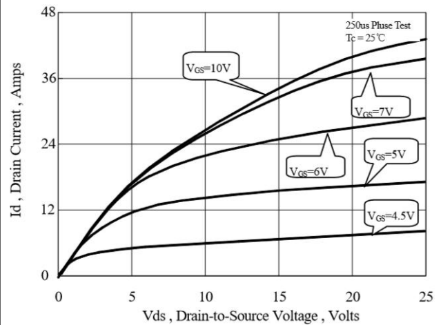
Figure 2. On-State Characteristics
