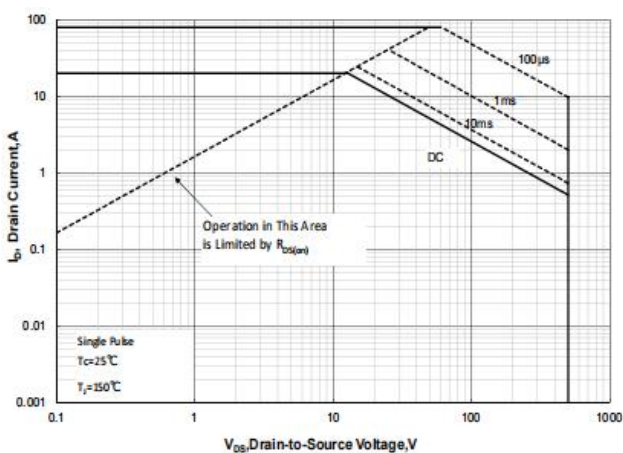
Figure 5. Maximum Forward Bias Safe Operating Area TO-220
