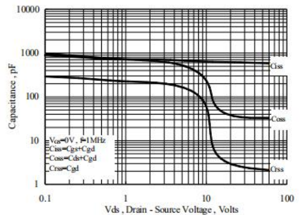
Figure 4. Capacitance Characteristics
