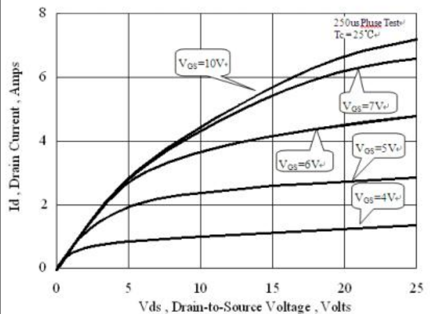
Figure 6. On-State Characteristics
