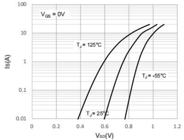
Figure 4. Body-Diode Characteristics
