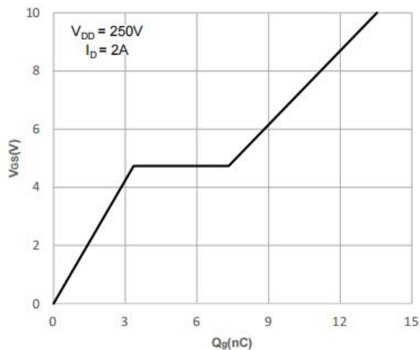
Figure 5. Gate-Charge Characteristics
