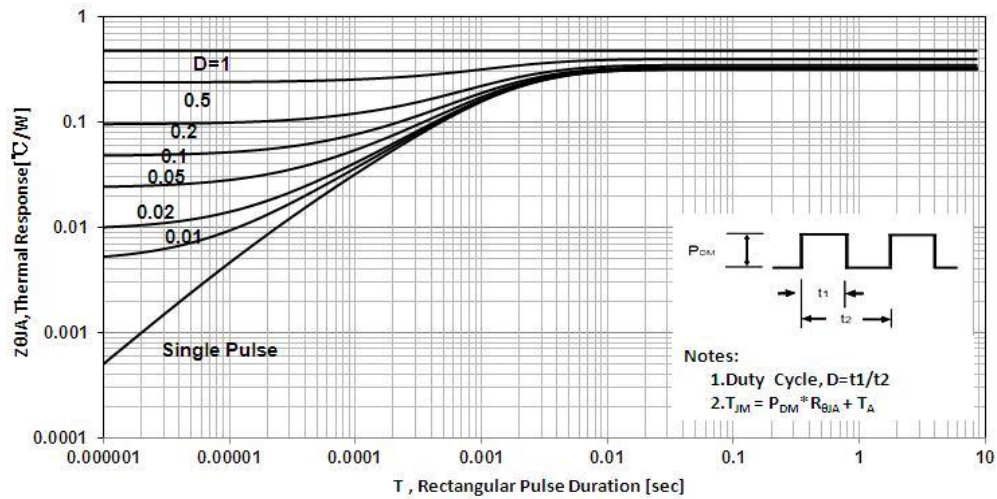
Figure 9. Normalized Effective Transient Thermal Impedance With Pulse Duration (TO-252)
