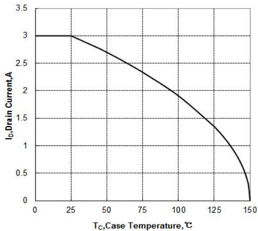
Figure 11. Maximum Continuous Drain VS Case Temperature
