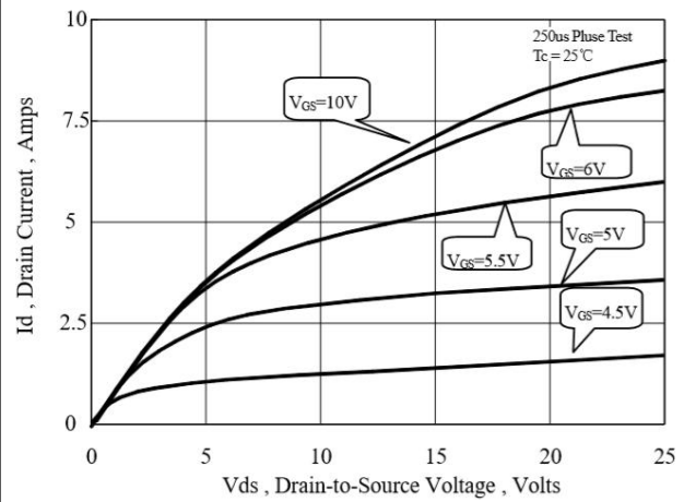
Figure 2. On-State Characteristics
