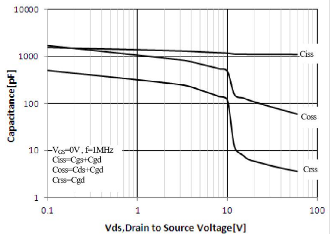
Figure 4. Capacitance Characteristics
