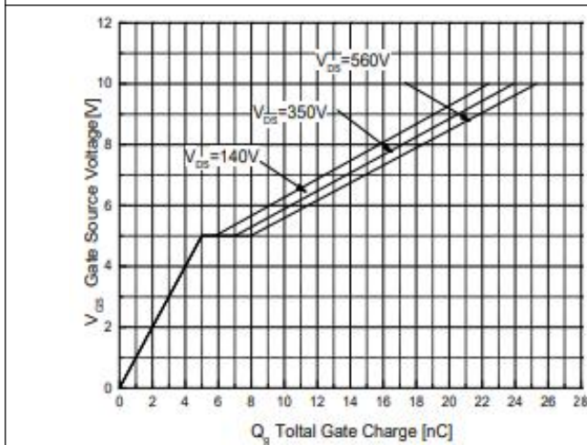
Figure 5. Gate-Charge Characteristics
