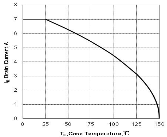
Figure 4. Maximum Drain Current with Case Temperature
