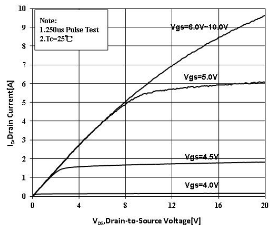
Figure 6. On-State Characteristics
