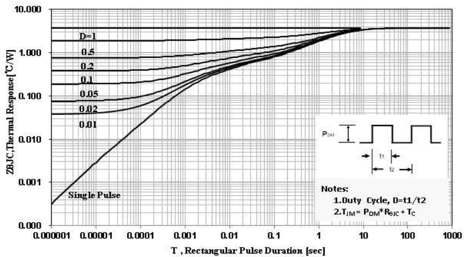
Figure 11. Normalized Effective Transient Thermal Impedance With Pulse Duration
