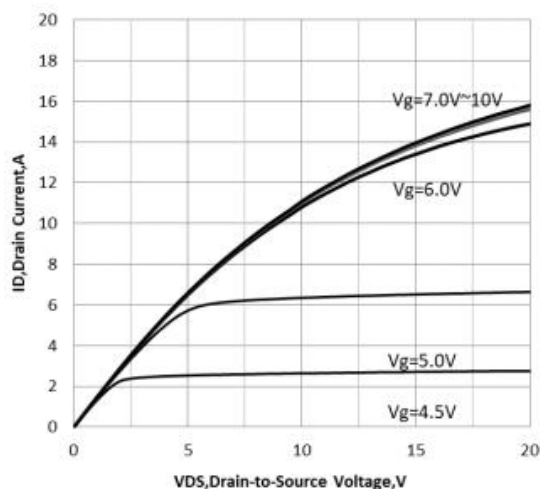
Figure 6. On-State Characteristics
