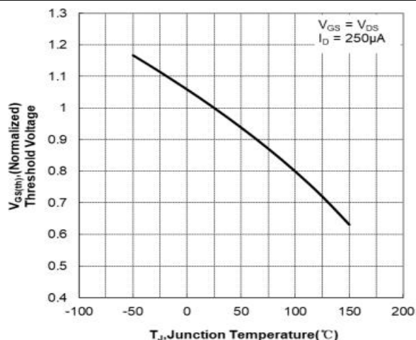
Figure 3. Typical Threshold Voltage vs Junction Temperature
