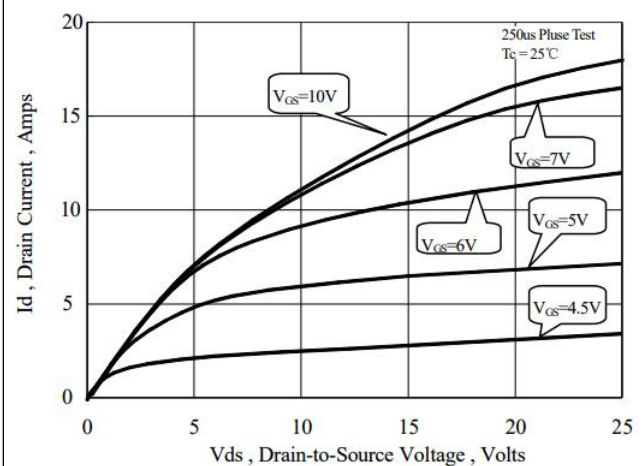
Figure 6. On-State Characteristics
