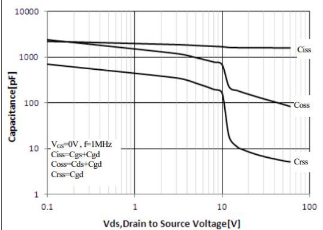
Figure 4. Capacitance Characteristics
