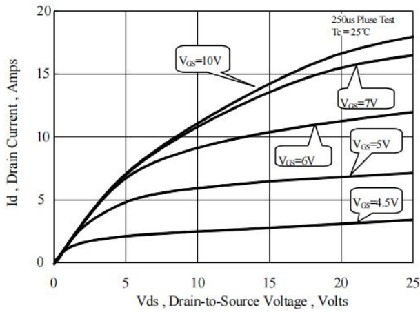
Figure1.On-State Characteristics
