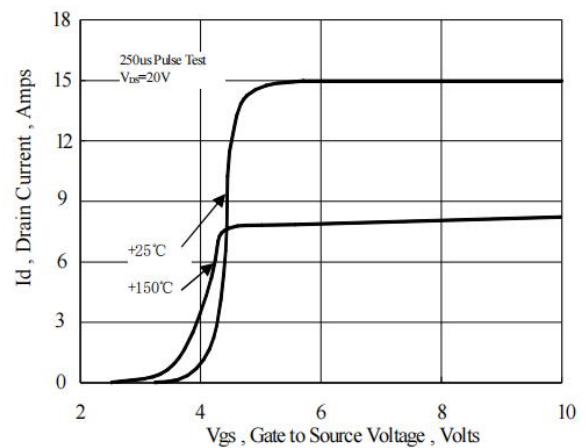
Figure 6. Transfer Characteristics Variation with Source Current
