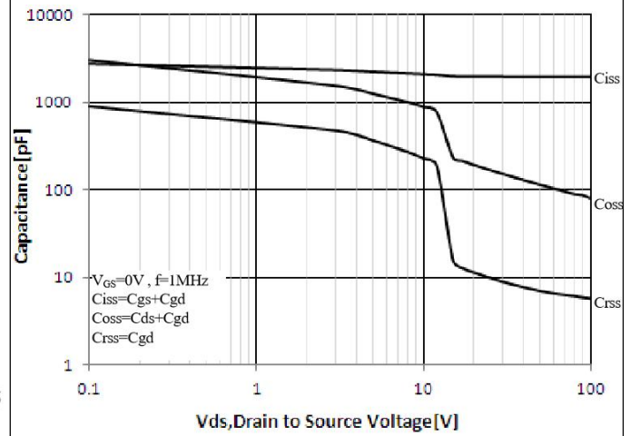
Figure 4. Capacitance Characteristics
