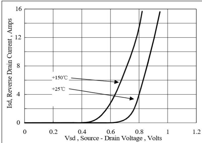
Figure 7. Body Diode Transfer Characteristics
