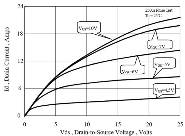
Figure 6. On-State Characteristics
