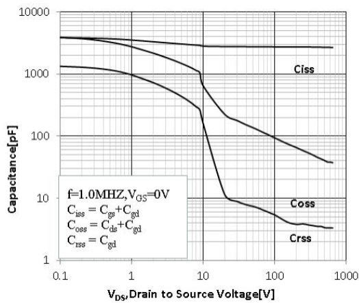
Figure 9. Capacitance Characteristics
