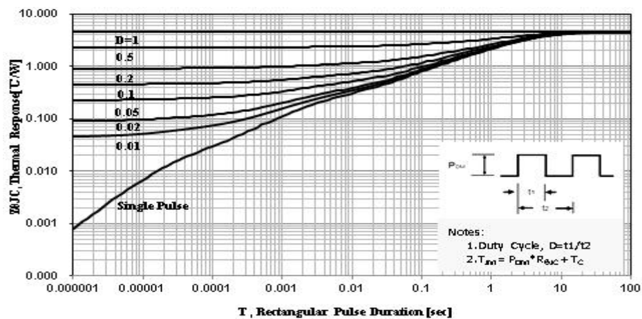
Figure 11. Normalized Effective Transient Thermal Impedance With Pulse Duration
