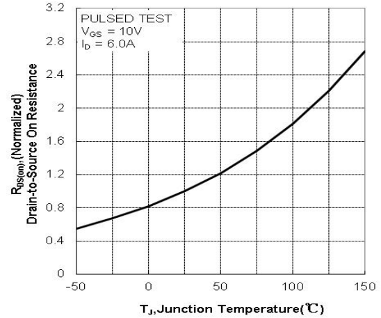
Figure 2. Normalized On-Resistance Variation with Temperature
