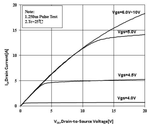
Figure 6. On-State Characteristics
