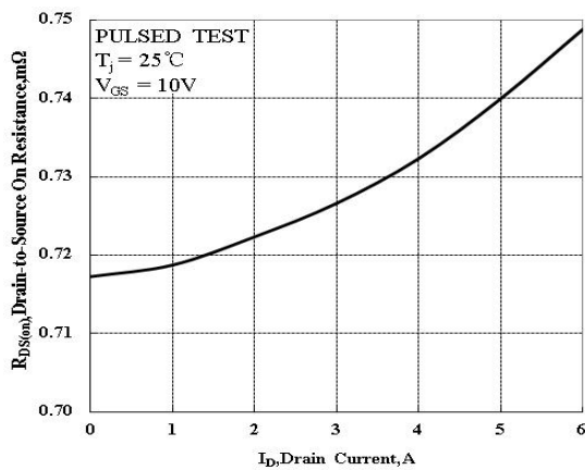
Figure 5. Typical Drain to Source ON Resistance vs Drain Current
