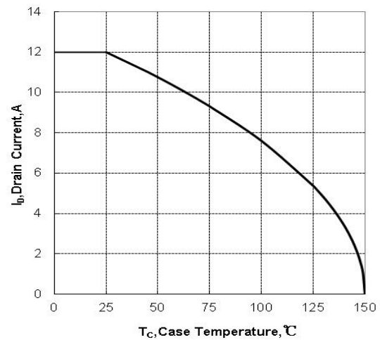
Figure 4. Maximum Drain Current with Case Temperature
