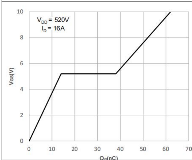
Figure 5. Gate-Charge Characteristics
