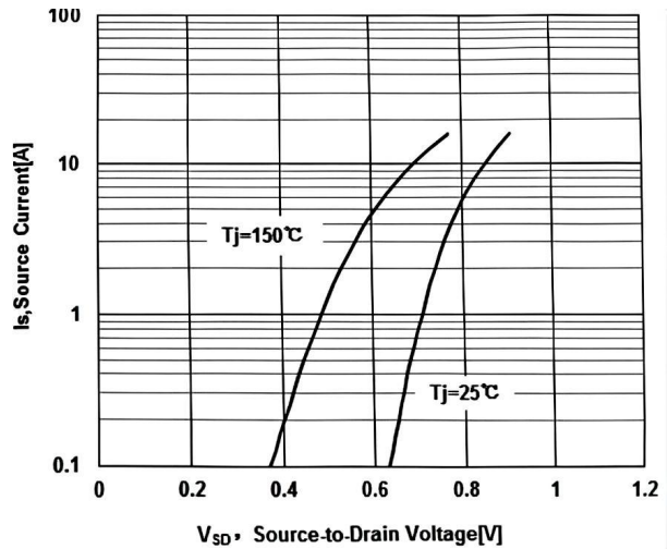
Figure 4. Body-Diode Characteristics
