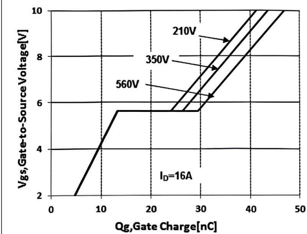
Figure 5. Gate-Charge Characteristics
