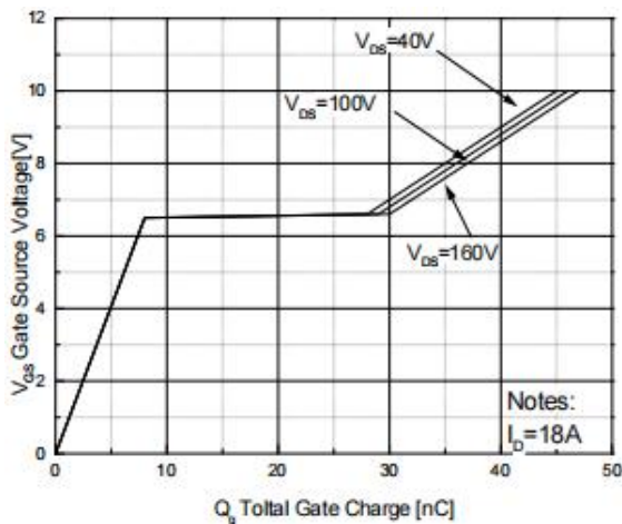
Figure 5. Gate-Charge Characteristics
