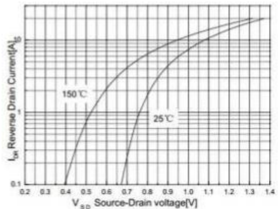
Figure 4. Body-Diode Characteristics
