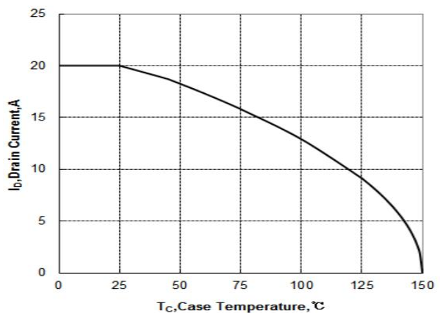
Figure 6. Maximum Continuous Drain Current vs Case Temperature
