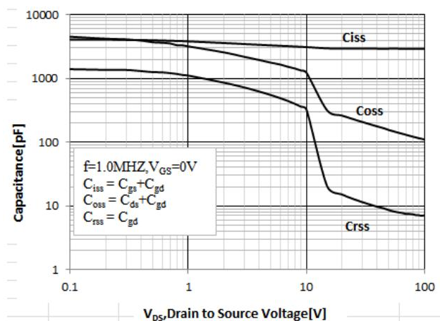
Figure 4. Typical Capacitance vs Drain to Source Voltage
