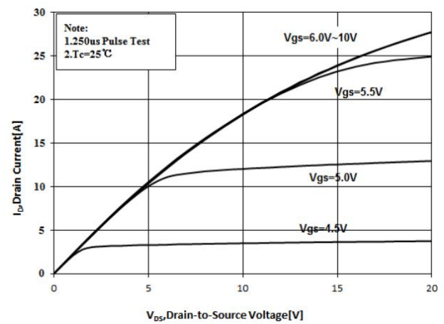
Figure 2. On-State Characteristics
