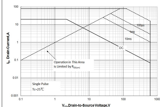
Figure 5 Maximum Forward Bias Safe Operating Area TO-220F
