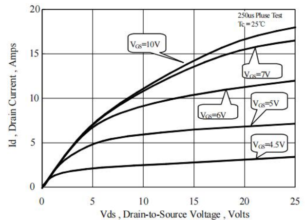
Figure 6. On-State Characteristics
