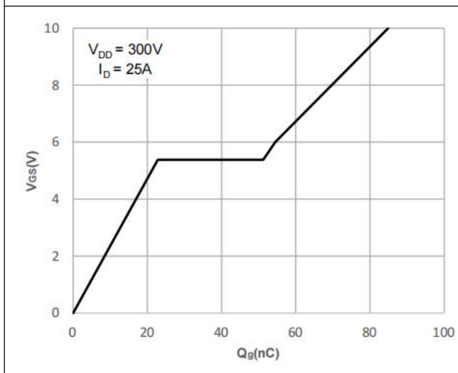
Figure 5. Gate-Charge Characteristics
