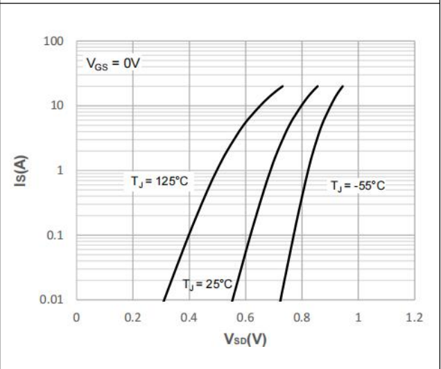
Figure 4. Body-Diode Characteristics
