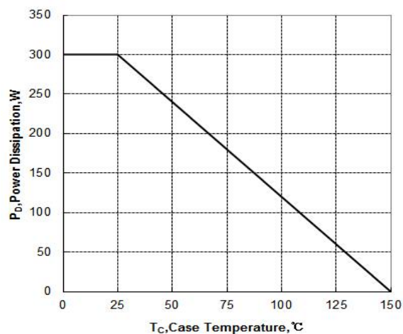
Figure 10: Maximum Power Dissipation vs Case Temperature
