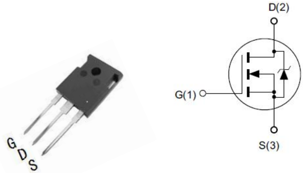
TO-247
