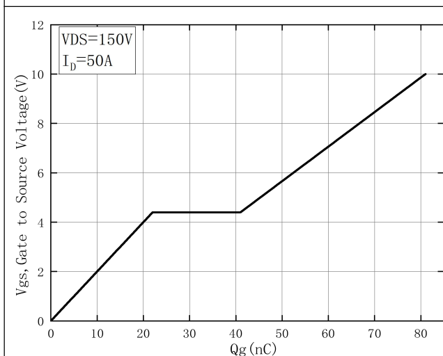
Figure 5. Gate-Charge Characteristics
