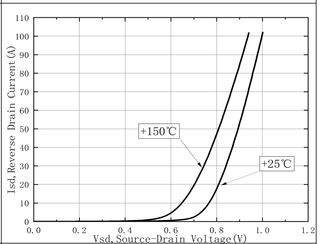
Figure 4. Body-Diode Characteristics
