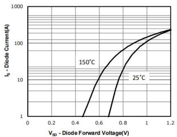
Figure 4. Body-Diode Characteristics
