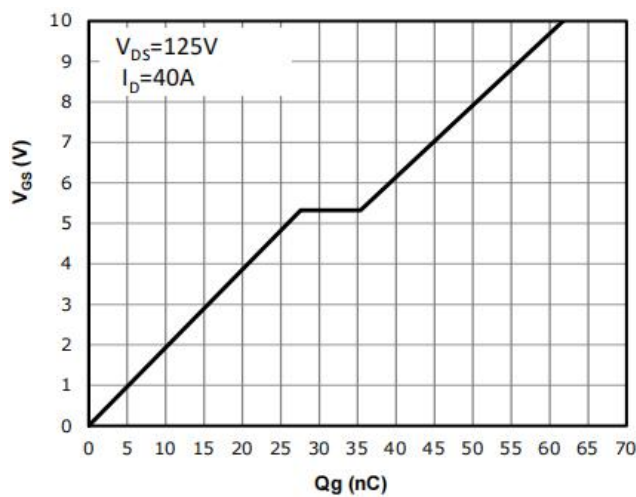
Figure 5. Gate-Charge Characteristics
