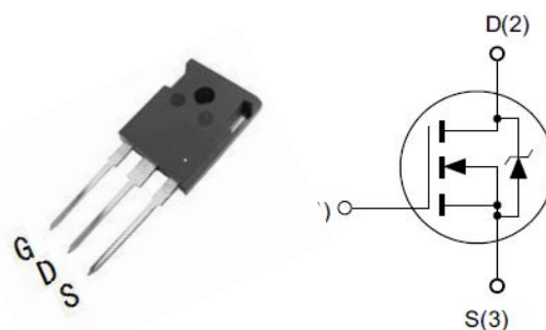
TO-247
