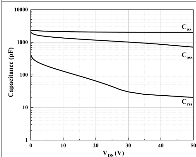
Figure 3. Typical Capacitance
