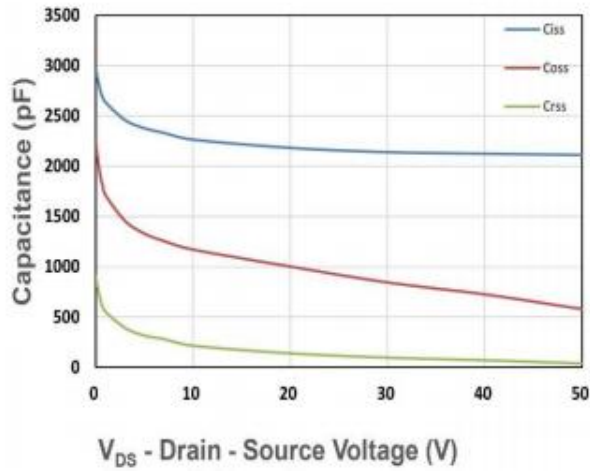
Figure 7. Capacitance
