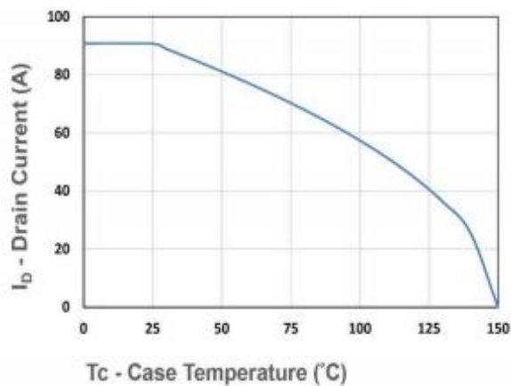
Figure11. Drain Current
