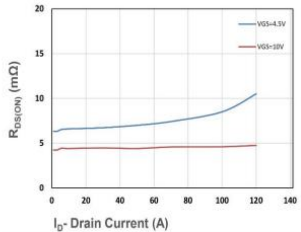
Figure 10. On-Resistance vs I_D
