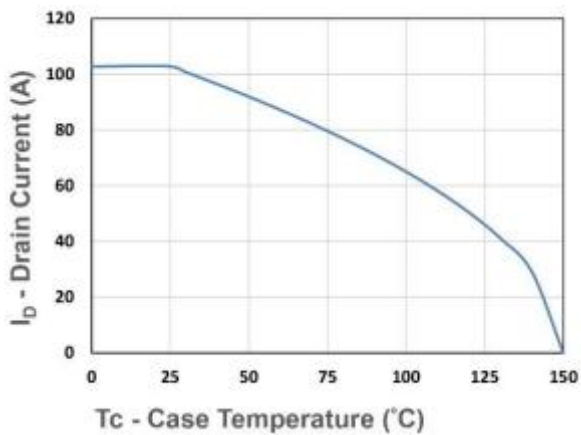
Figure 11. Drain Current
