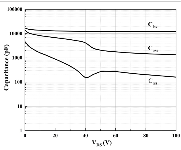
Figure 4. Typical Capacitance
