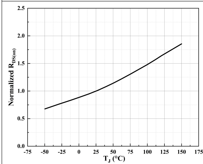
Figure 9. Normalized Static Drain-Source On-Resistance vs. Junction Temperature
