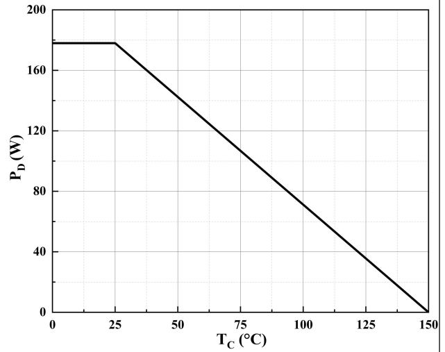
Figure 8. Maximum Power Dissipation vs. Case Temperature
