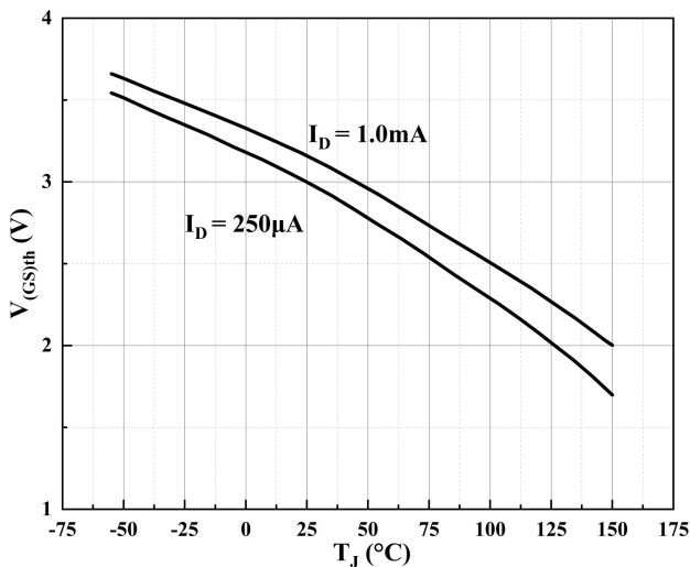
Figure 11. Gate Threshold Voltage vs. Junction Temperature
