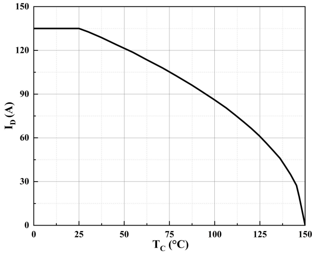
Figure 7. Maximum Continuous Drain Current vs. Case Temperature
