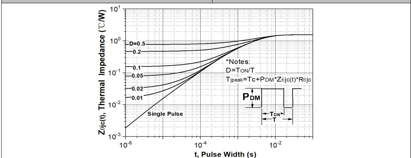
Figure 11. Transient Thermal Impedance
