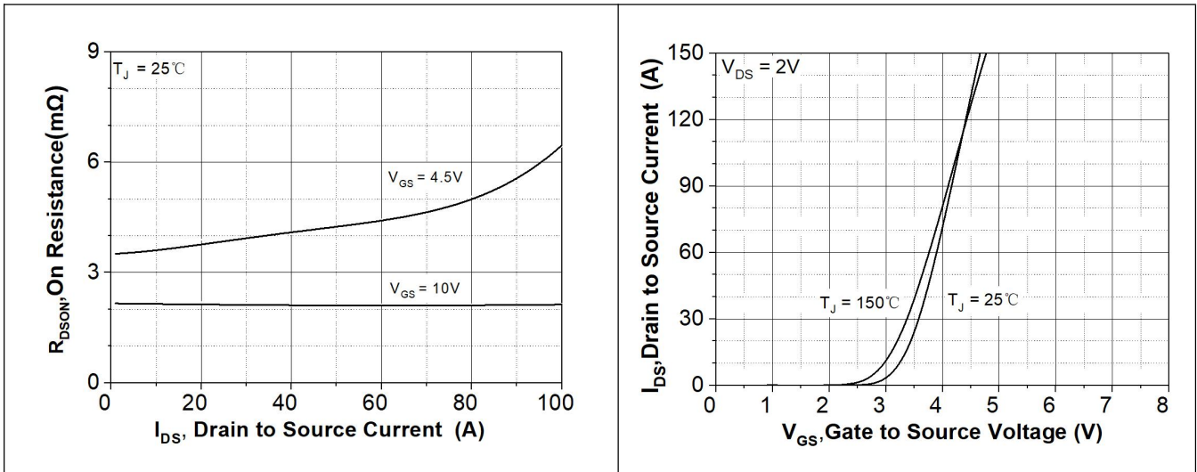
Figure 7. Drain-Source On-State Resistance
