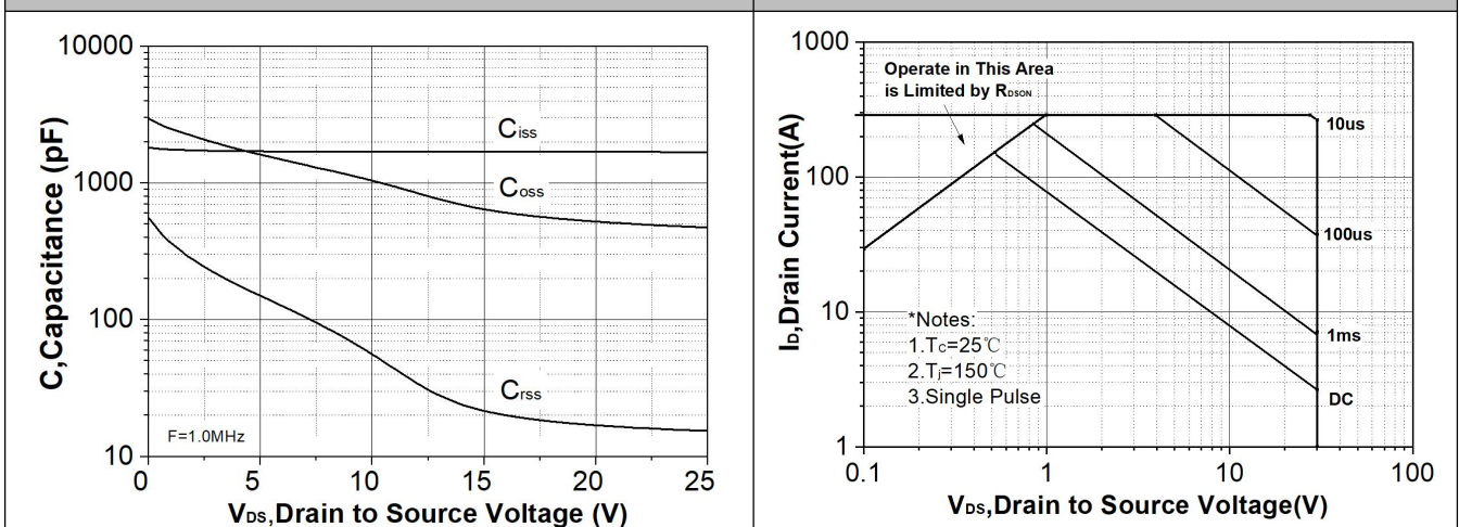
Figure 9. Capacitance
