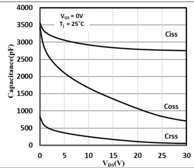
Figure 4. Typical Capacitance
