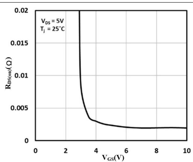
Figure 6. On-Resistance vs Gate Voltage
